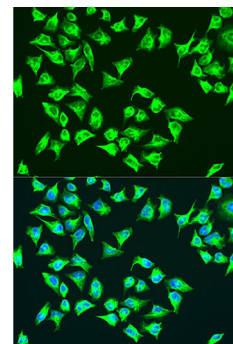
Fig. 2. Immunofluorescence analysis of U2OS cells using ATP6 antibody at dilution of 1:100. Blue: DAPI for nuclear staining.
