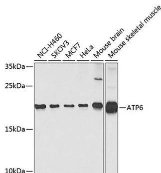
Fig. 1. Western blot analysis of extracts of various cell lines, using ATP6 antibody at 1:1000 dilution. Secondary antibody: HRP-labeled Goat Anti-Rabbit IgG(H+L) (A0208) at 1:1000 dilution. Lysates/proteins: 25μg per lane. Blocking buffer: QuickBlock™ Blocking Buffer (P0231). Detection: BeyoECL Star (P0018A). Exposure time: 1s.
